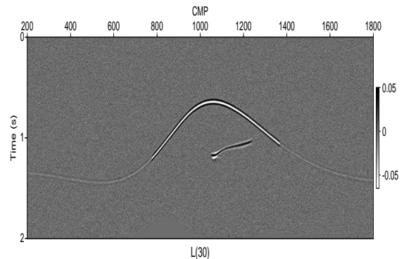
Figure 4: Four different attributes for the synthetic model depicted in Figure 3: (A + B) / 2 , A \times B , Fluid Factor \Delta F , and L(30^\circ) .
