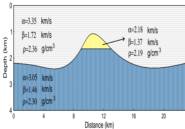
Figure 3: Synthetic model for the experiments: a shale layer over a brine-sand dome, with a small layer of gas-sand in the top.
