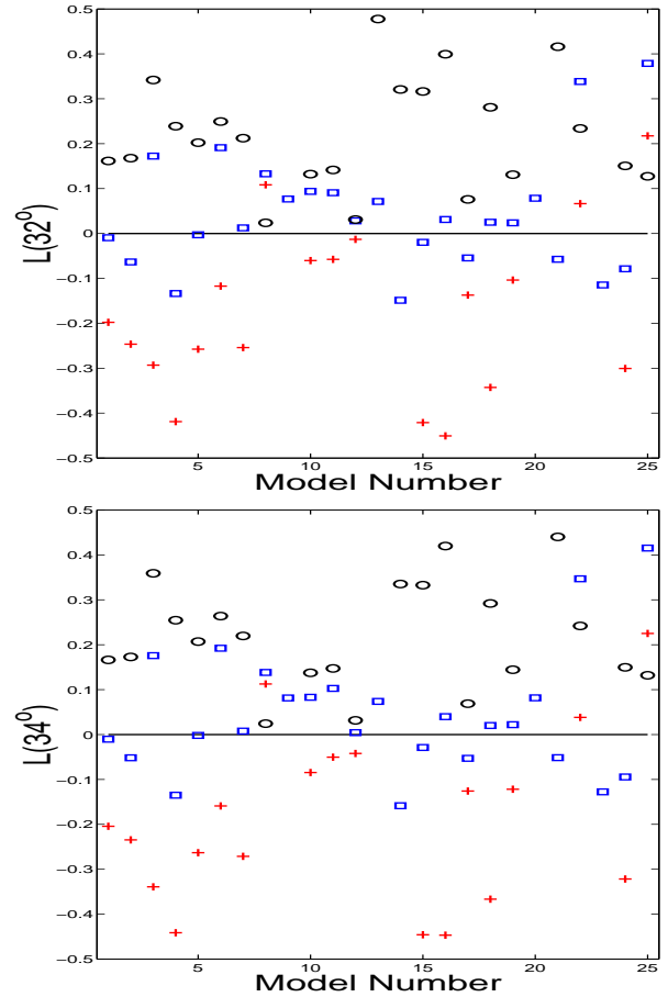
Figure 2: Impedande-type indicator L for five diferent values of \theta near 30^\circ for 25 measurements of shale over brine-sand ( \square ), shale over gas-sand ( + ) and gas-sand over brine-sand ( \circ ).
