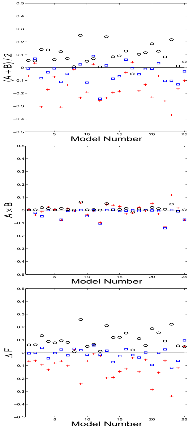
Figure 1: Three different attributes for 25 measurements of shale over brine-sand ( \square ), shale over gas-sand ( + ) and gas-sand over brine-sand ( \circ ): (A + B) / 2 , A \times B , and Fluid Factor \Delta F .
